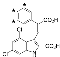
Figure 1. Structure of [\text{}^3\text{H}]\text{MDL-105,519} , positions of the tritium atoms are indicated by asterisks.
